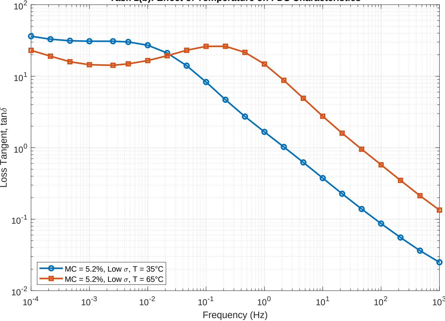
Task 1(b): Effect of Temperature on FDS Characteristics
